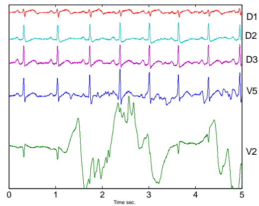
Figure 11: Detail of ECG signals during abduction-adduction of the left shoulder
