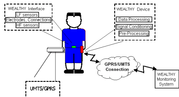
Fig. 1: Overview of WEALTHY system
