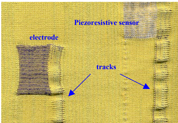
Fig. 2: Particular of WEALTHY interface
